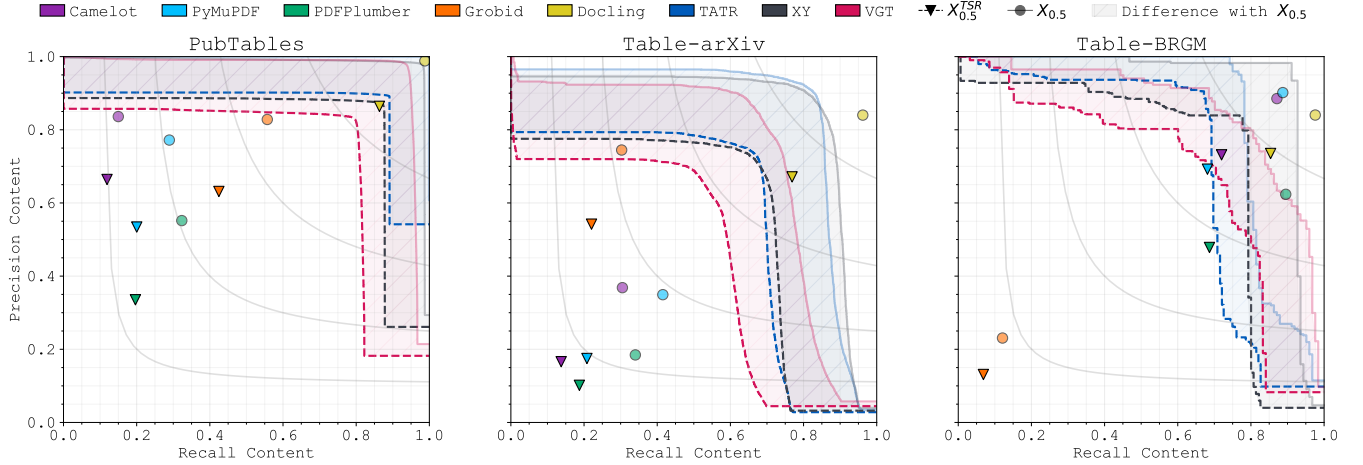
Figure 16: p^{\text{Con}} - R^{\text{Con}} curves for (left to right): PubTables, Table-arXiv dataset and Table-BRGM ( bbox TD).
