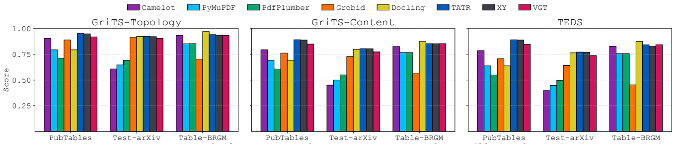
Figure 15: TSR results for GriTS Topology, GriTS Content and TEDS ( bbox evaluation).
