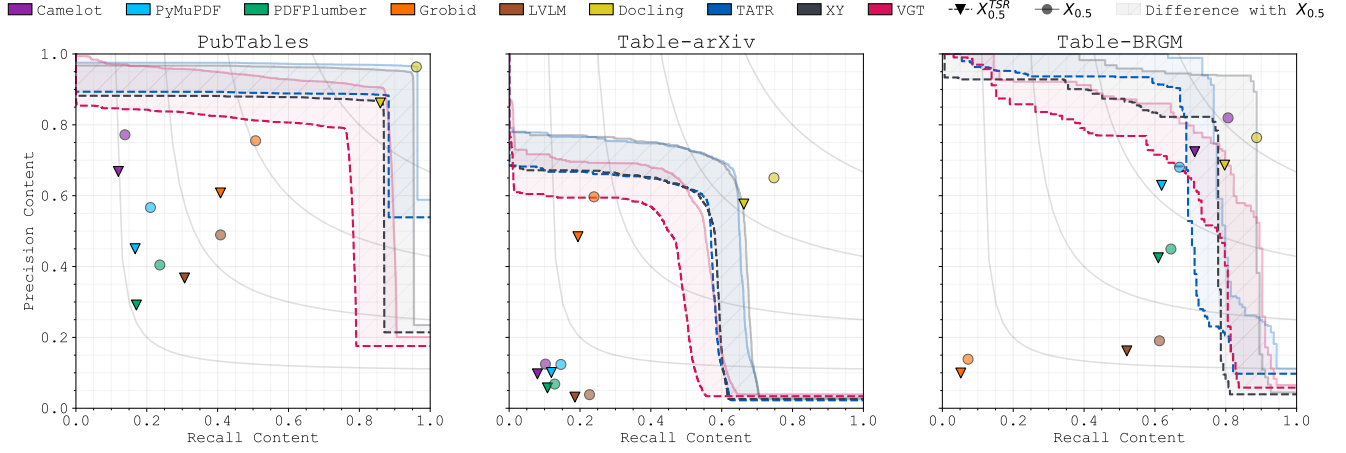
Figure 18: p^{\text{Con}} - R^{\text{Con}} curves for (left to right): PubTables, Table-arXiv dataset and Table-BRGM ( content TD).
