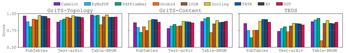
Figure 7: TSR_{TL} for GriTS Topology, GriTS Content and TEDS ( content evaluation). Scores are between 0.5 and 1.
