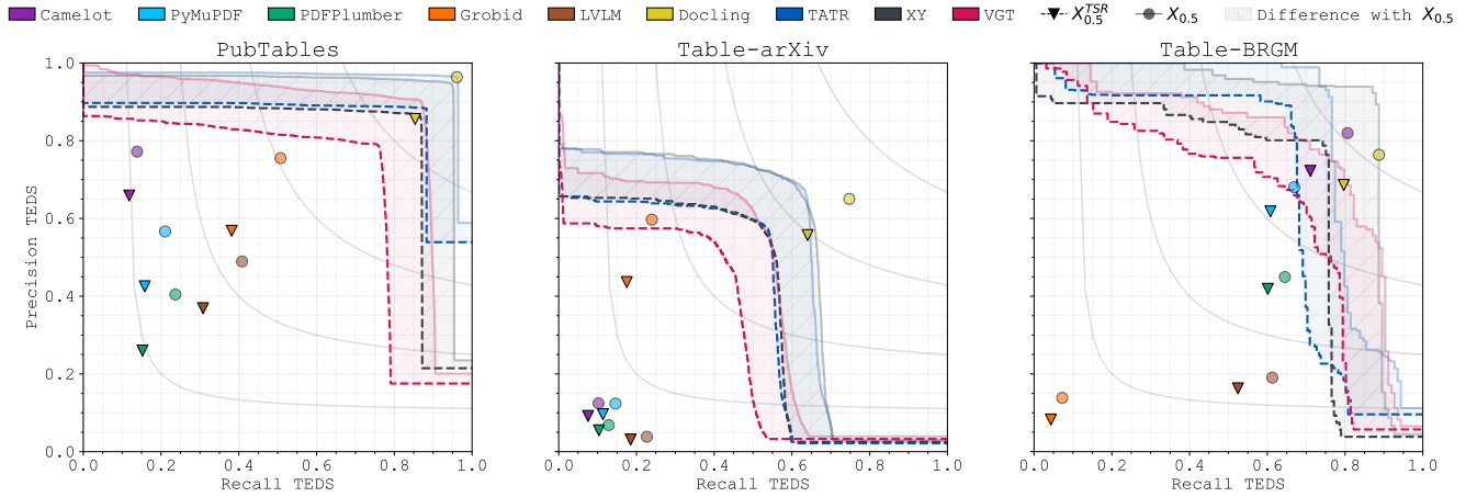
Figure 19: p^{\text{TEDS}} - R^{\text{TEDS}} curves for (left to right): PubTables, Table-arXiv dataset and Table-BRGM ( content TD).
