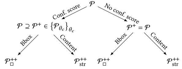
Figure 3: TSR inputs depending on the TD model type (with or without a confidence score), and evaluation type (bbox-based or content-based).
