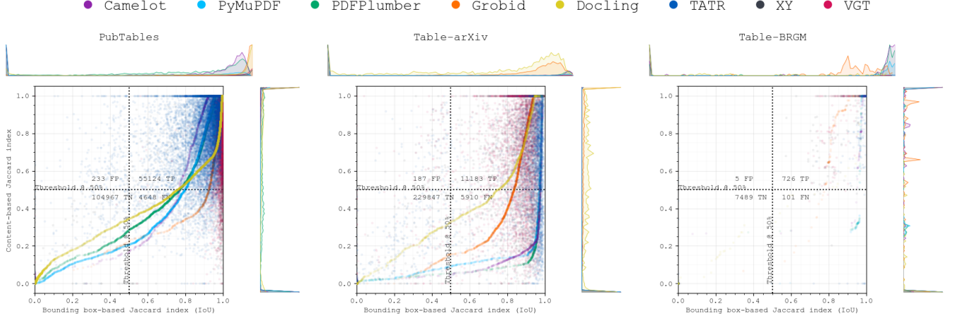
Figure 14: Content Jaccard index distribution over bounding box Jaccard index (IoU) distribution for (left to right): PubTables, Table-arXiv dataset and Table-BRGM.
