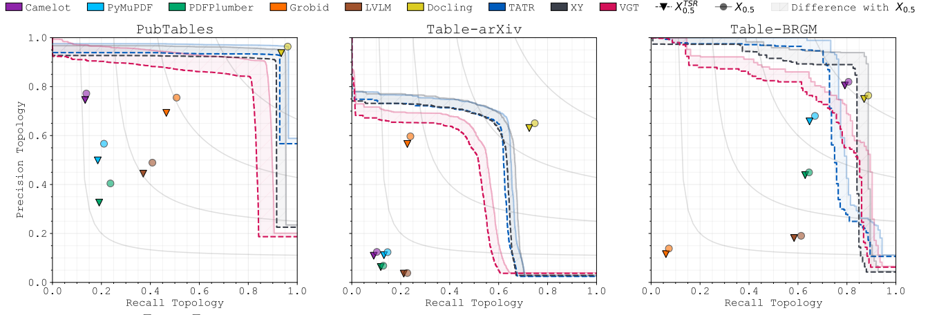
Figure 17: p^{\text{Top}} - R^{\text{Top}} curves for (left to right): PubTables, Table-arXiv dataset and Table-BRGM ( content TD).
